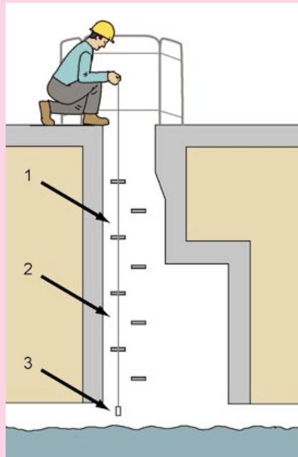
Air monitoring should be conducted at different levels of a manhole.
